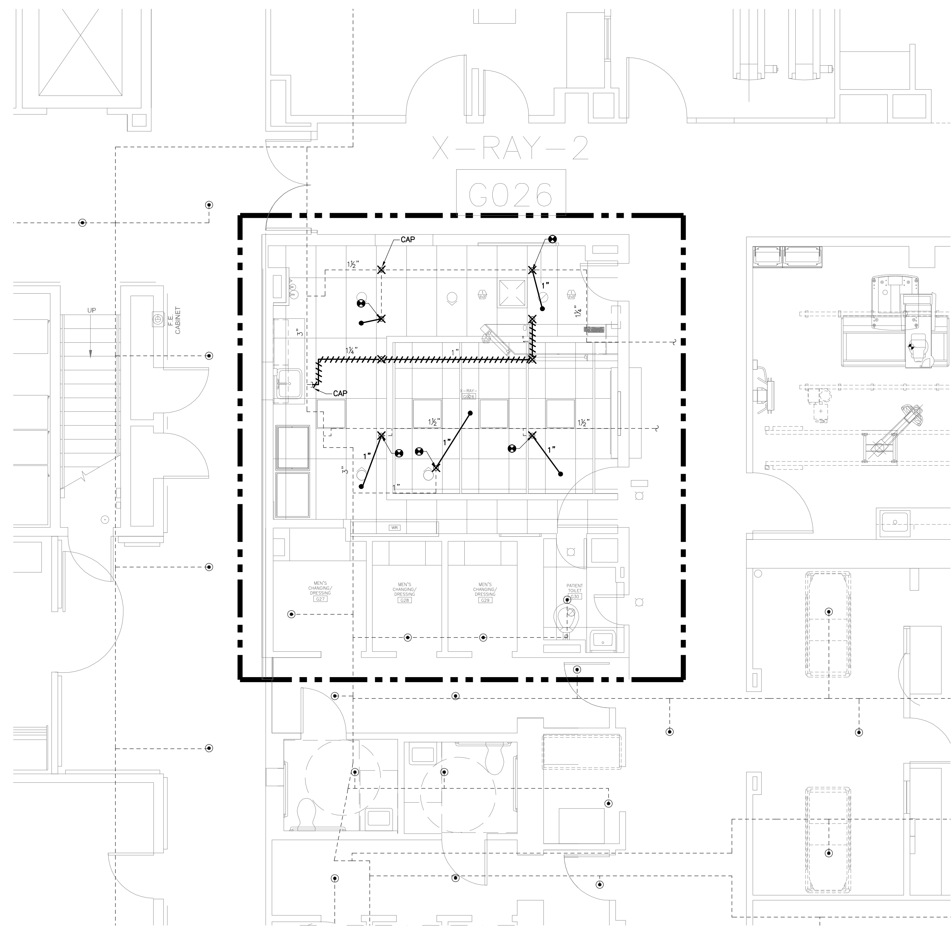
XRAY-2 ROOM PART PLAN SCALE: 1/4"=1'-0"
