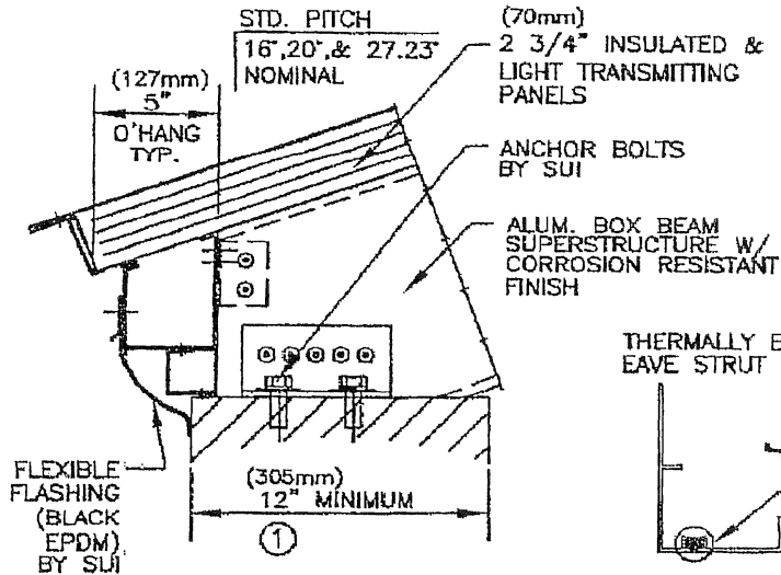
TYPICAL HIP-ROOF
