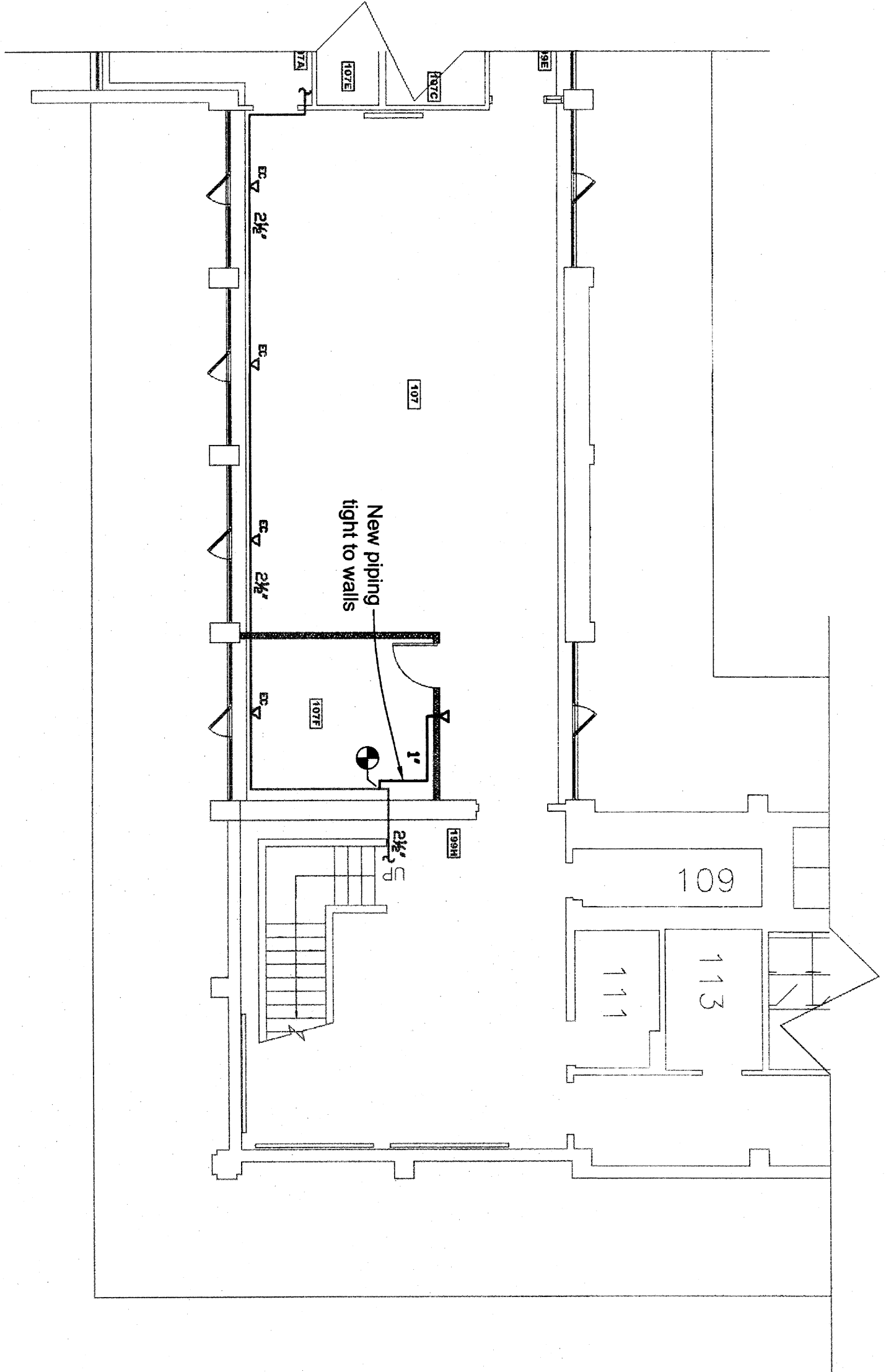
First Floor - New Fire Protection Plan SCALE: 1/8" = 1' 0"
