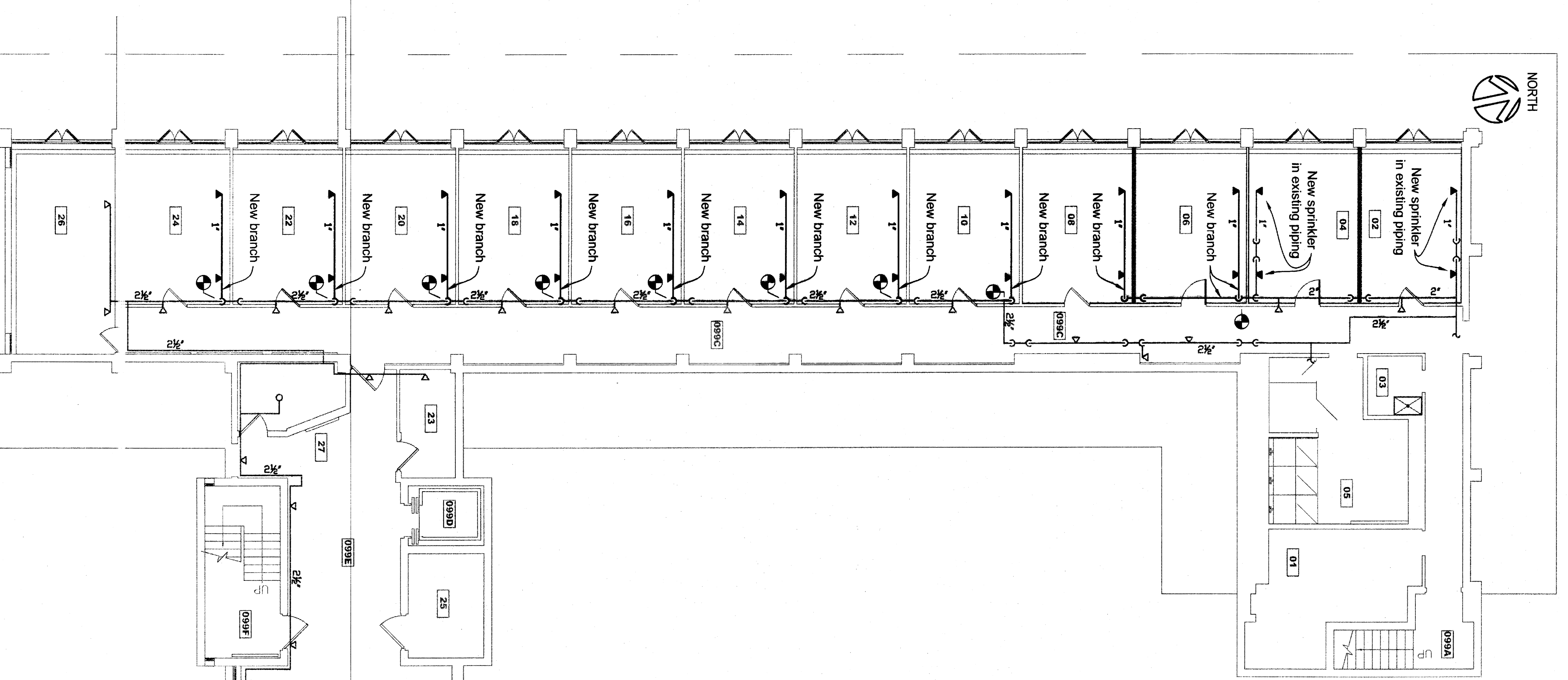
Basement Floor - New Fire Protection Plan SCALE: 1/8" = 1' 0"
