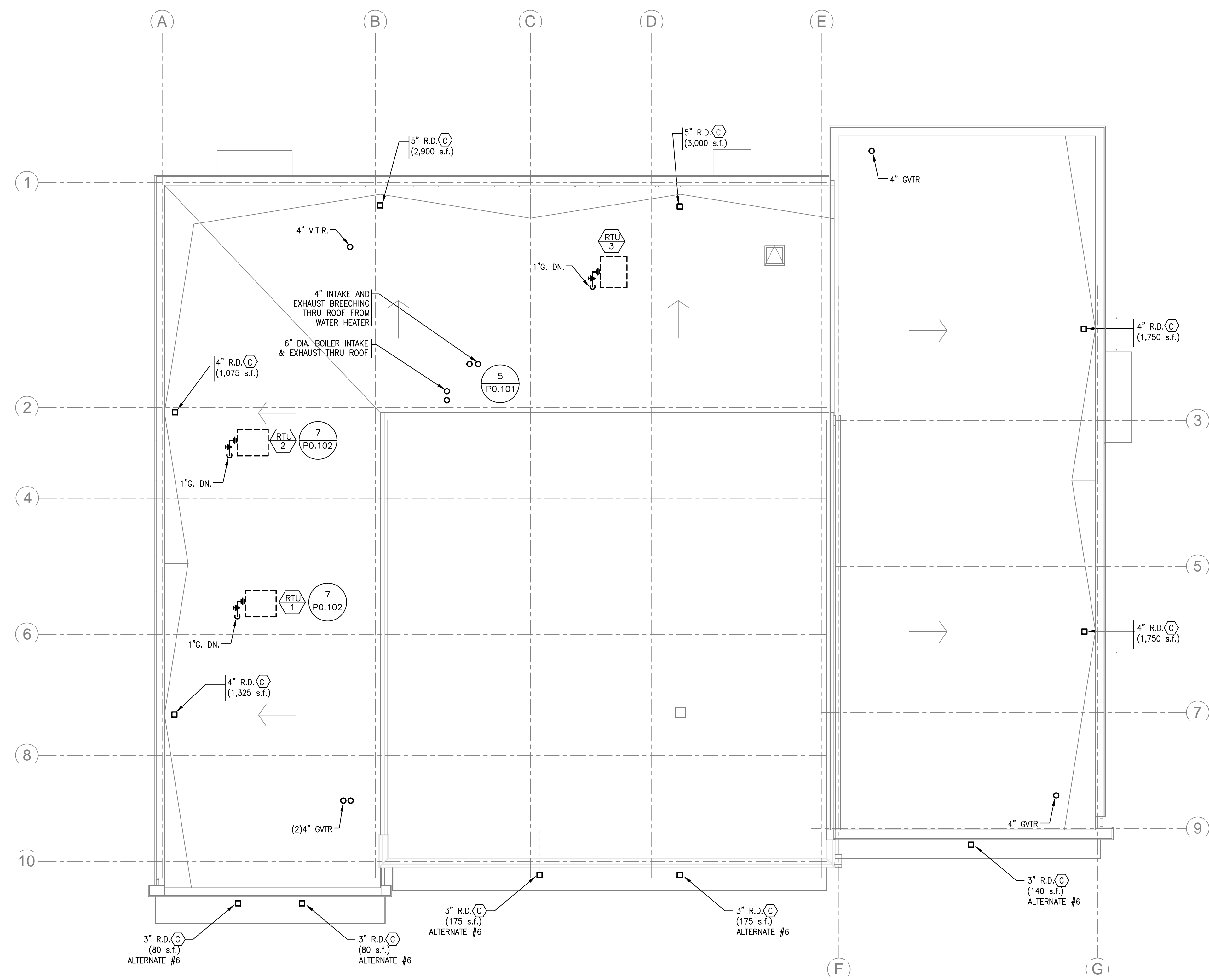
1 ROOF PLAN -- PLUMBING SCALE: 1/8" = 1'-0"
