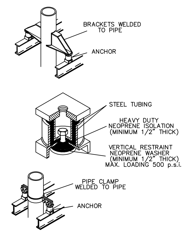
ADA ALL DIRECTIONAL ANCHOR SPECIFICATION 25
