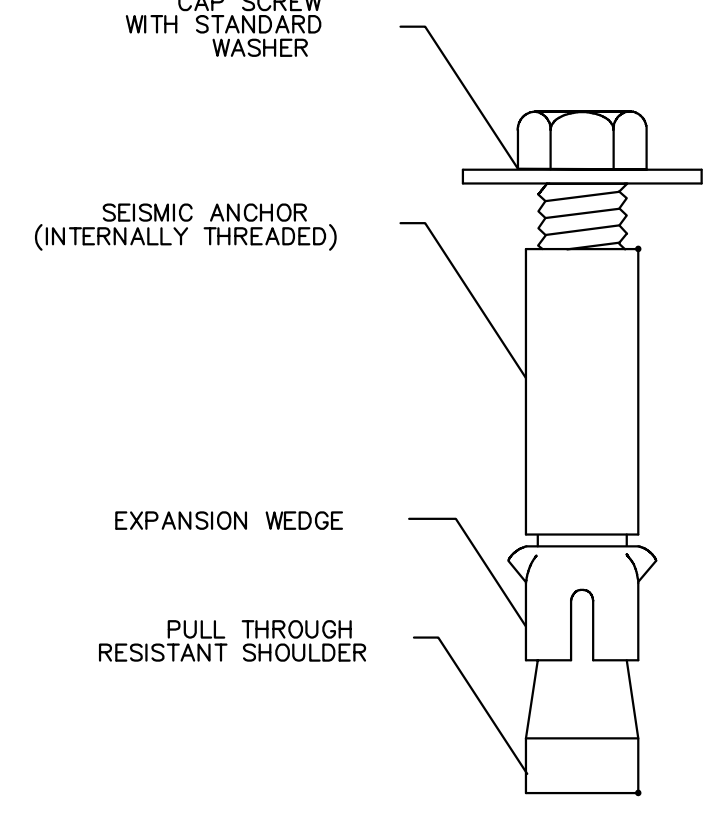
SAB SEISMIC ANCHOR BOLT SPECIFICATION 19
