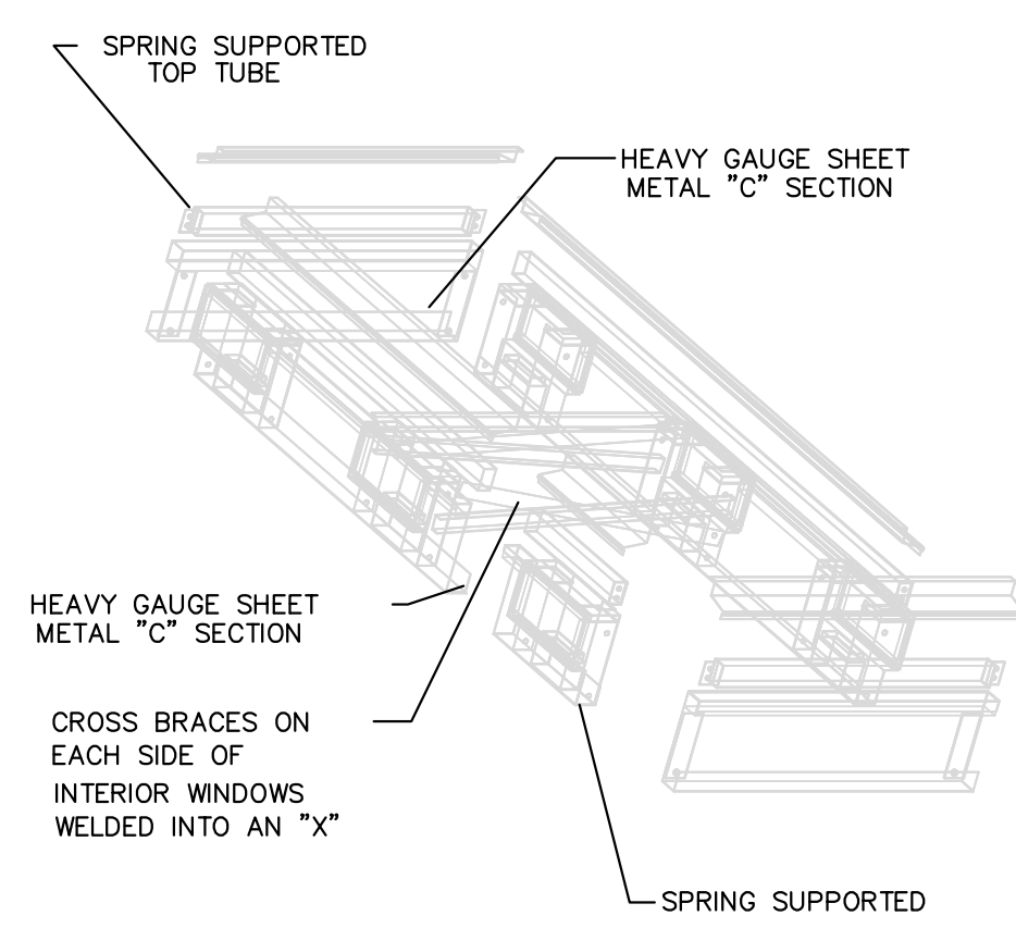
RSC SEISMIC ROOFTOP CURB SPECIFICATION 22
