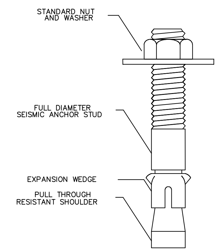
SAS SEISMIC ANCHOR STUD SPECIFICATION 18
